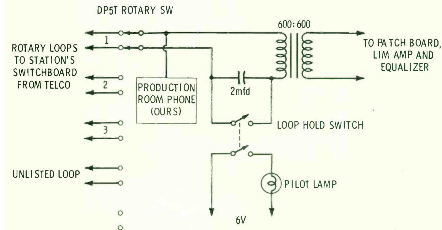
Fig. 2 Wiring at the station.
